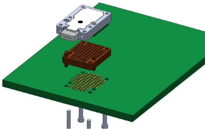
LightVISION LGA interposer and board attachment.
