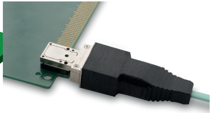
Cable assembly with rubber boot connected to LightSNAP interface.
