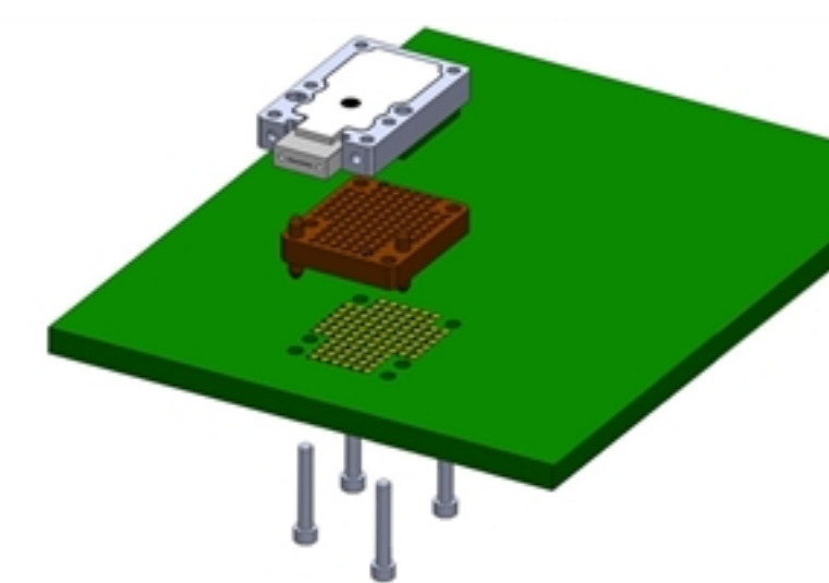
LightVISION industrial optical module with robust screw-in electrical interface
